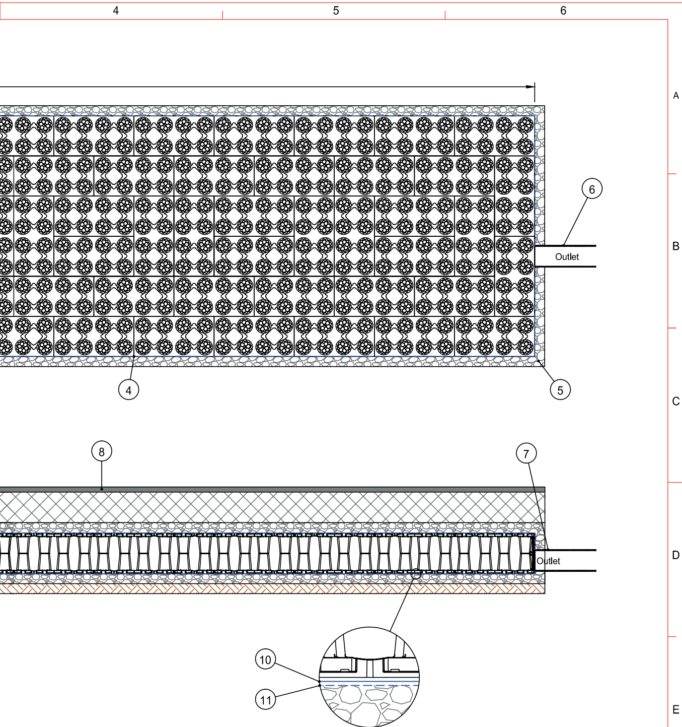
Detail A
